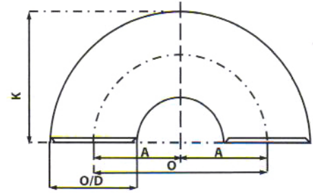
180° LR RETURN / U BEND
