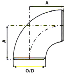
90° SR ELBOW
